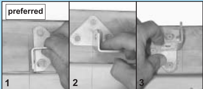
FIG. 2-5 Header bracket in place (3 methods).
