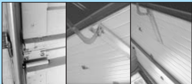
FIG. 2-6 Examples of door bracing.
