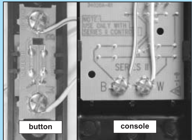
FIG. 5-2 Wall control wire attachment.
