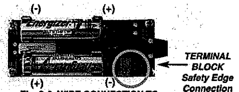
Fig. 2-6 WIRE CONNECTION TO TERMINAL BLOCK
