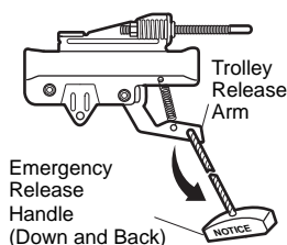
LOCKOUT POSITION
